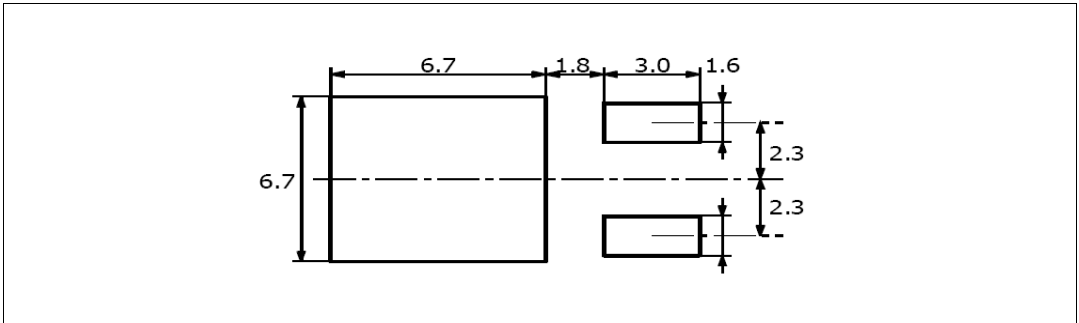
Figure 30. DPAK footprint
